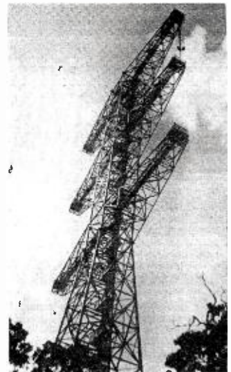
W2XMN, the Armstrong frequency modulated station, is operating from this antenna atop the Palisades on the Hudson. The tower, 400 feet high and with 150-foot crossarms, can be seen from Riverside Drive, Manhattan.
