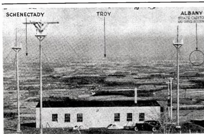
HERE is the new GE 10 kw. television transmitting station in the Belderberg Mountains, New York, with Schenectady, Troy and Albany barely discernible in the distance. The district has a population of some 500,000. Tower at left supports the receiving antenna, picking up signals radioed from Schenectady; the next tower will broadcast the televised pictures and the one at the right will broadcast voice. Adjoining the voice antenna are power line poles coming up the mountainside.
